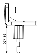
UK plug part no. 018112 Weight: 30g
